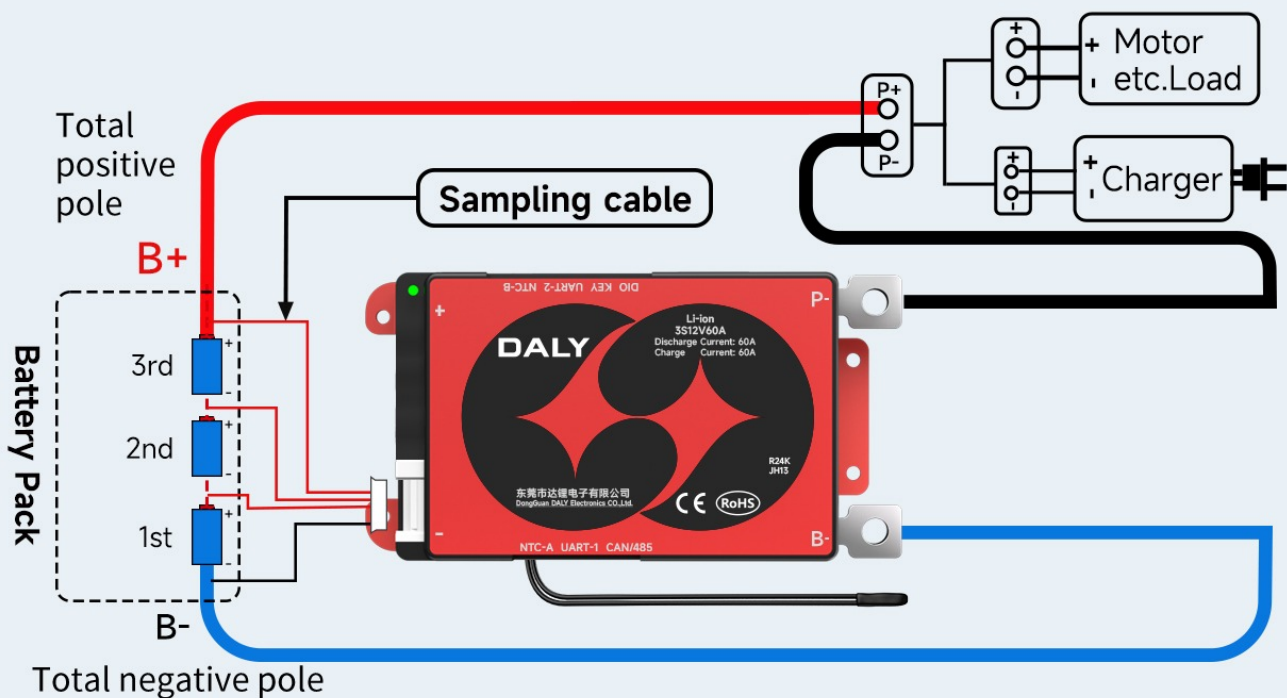
(Wiring Diagram) ⤴
